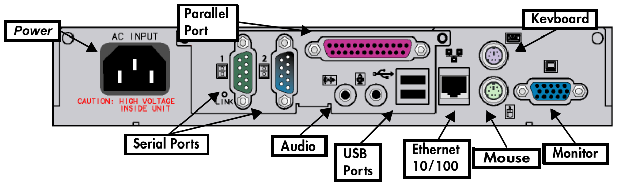
Capio II back panel
