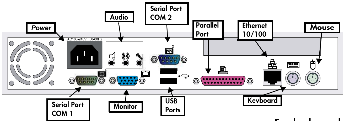
Eon back panel
