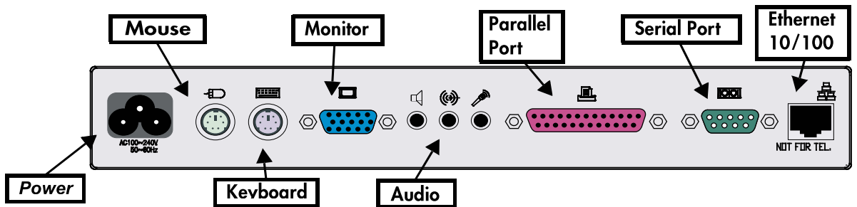
Capio 600 back panel
